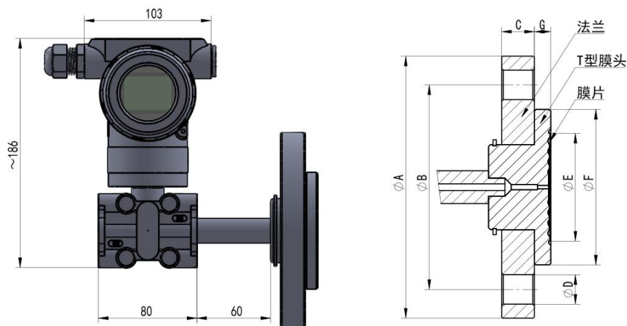
Flange and diaphragm dimension drawing
